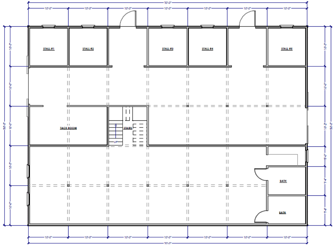
Main Level
